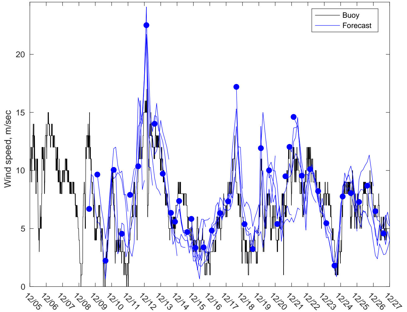
NDBC 44020 vs GFSWinds: 3 to 5 day forecast
