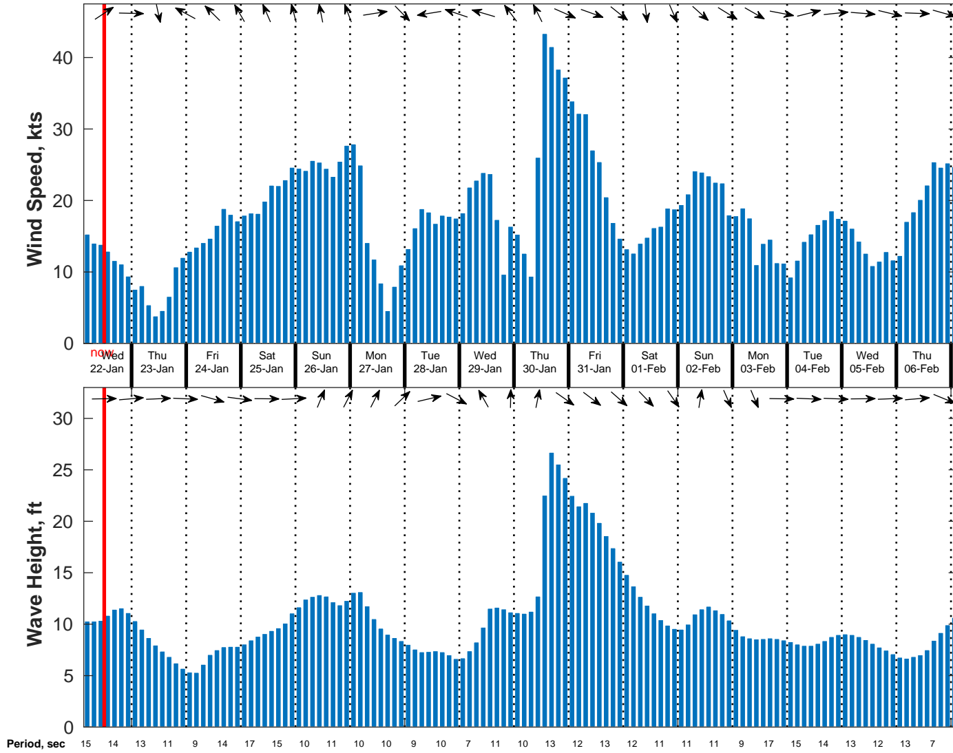
Wind & Wave Forecast for NDBC 46246 from 22-Jan-2025 03:00:00 to 07-Feb-2025 03:00:00
