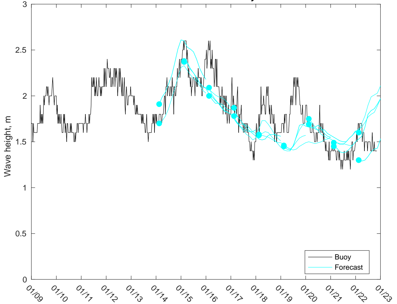
NDBC 52211 vs CMEMSWaves: 5 to 7 day forecast
