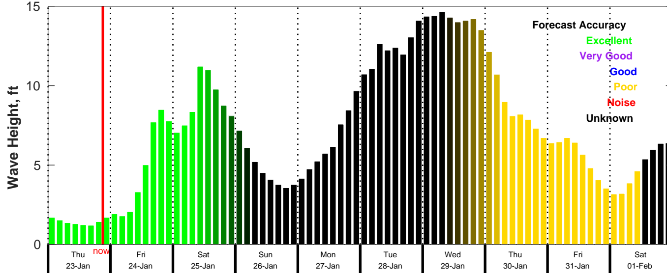
CMEMS Wave Forecast for NDBC 62305 from 22-Jan-2025 00:00:00 to 01-Feb-2025 00:00:00
