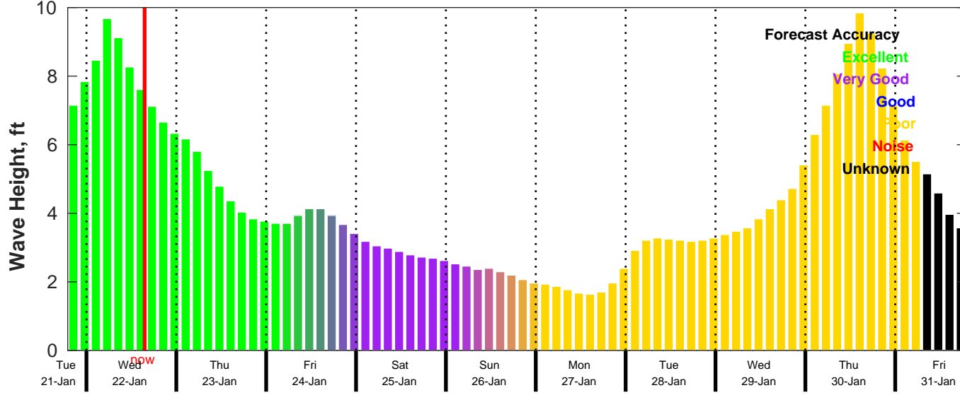
CMEMS Wave Forecast for NDBC 41013 from 21-Jan-2025 19:00:00 to 31-Jan-2025 19:00:00
