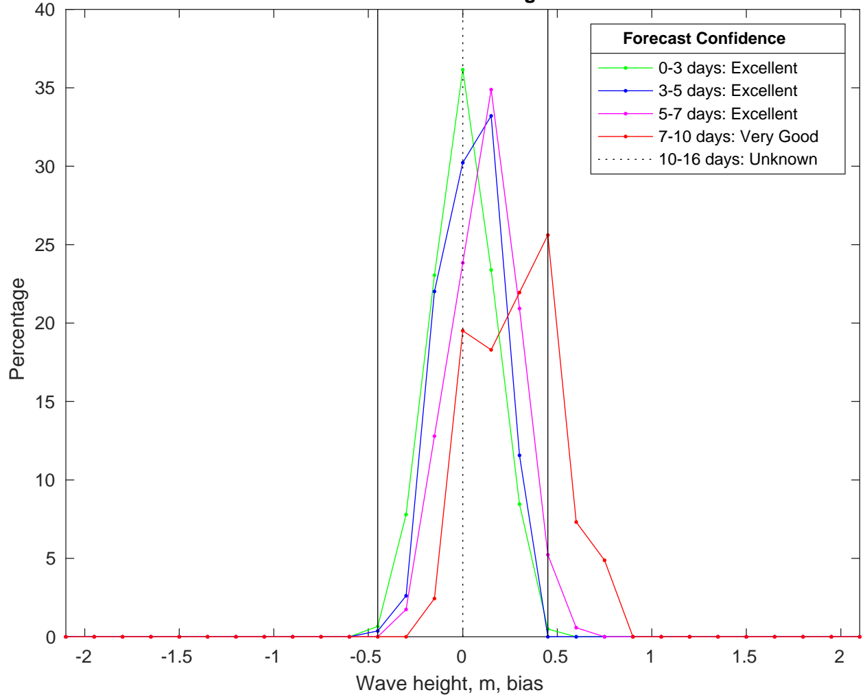
NDBC 41040 vs CMEMSWaves Bias Histogram: 22-Jan-2025
