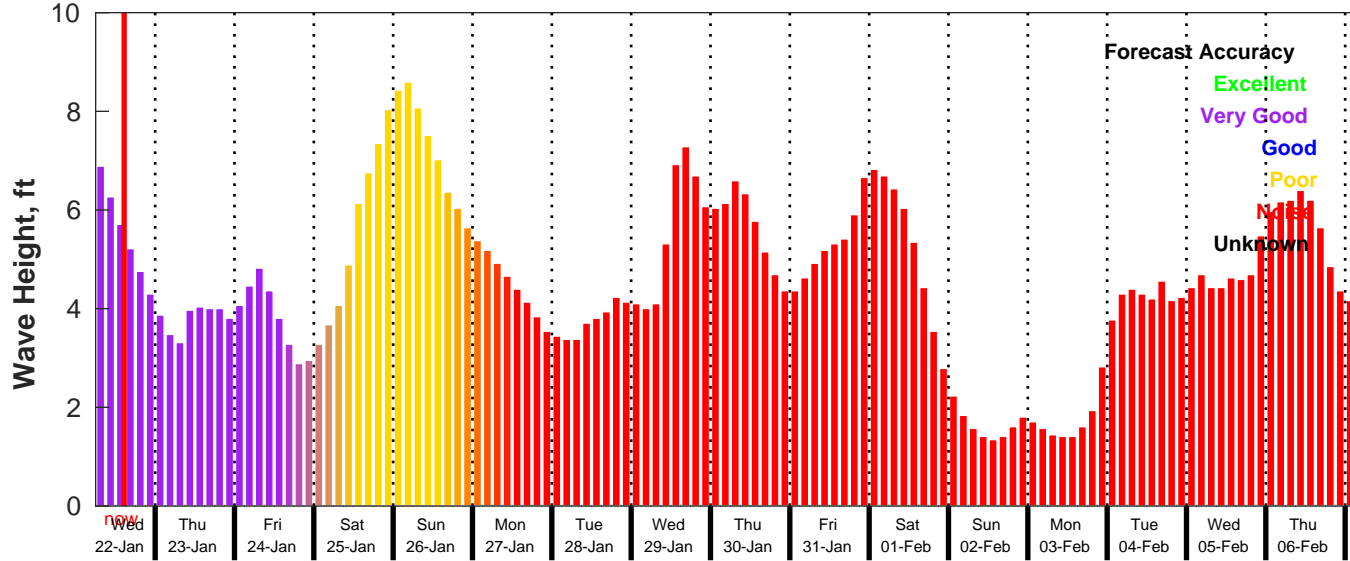
GFS Wave Forecast for NDBC 42020 from 22-Jan-2025 06:00:00 to 07-Feb-2025 06:00:00
