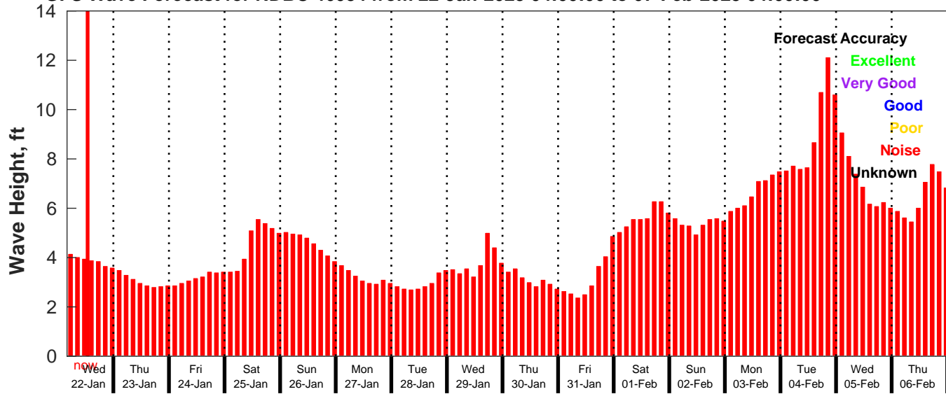
GFS Wave Forecast for NDBC 46054 from 22-Jan-2025 04:00:00 to 07-Feb-2025 04:00:00
