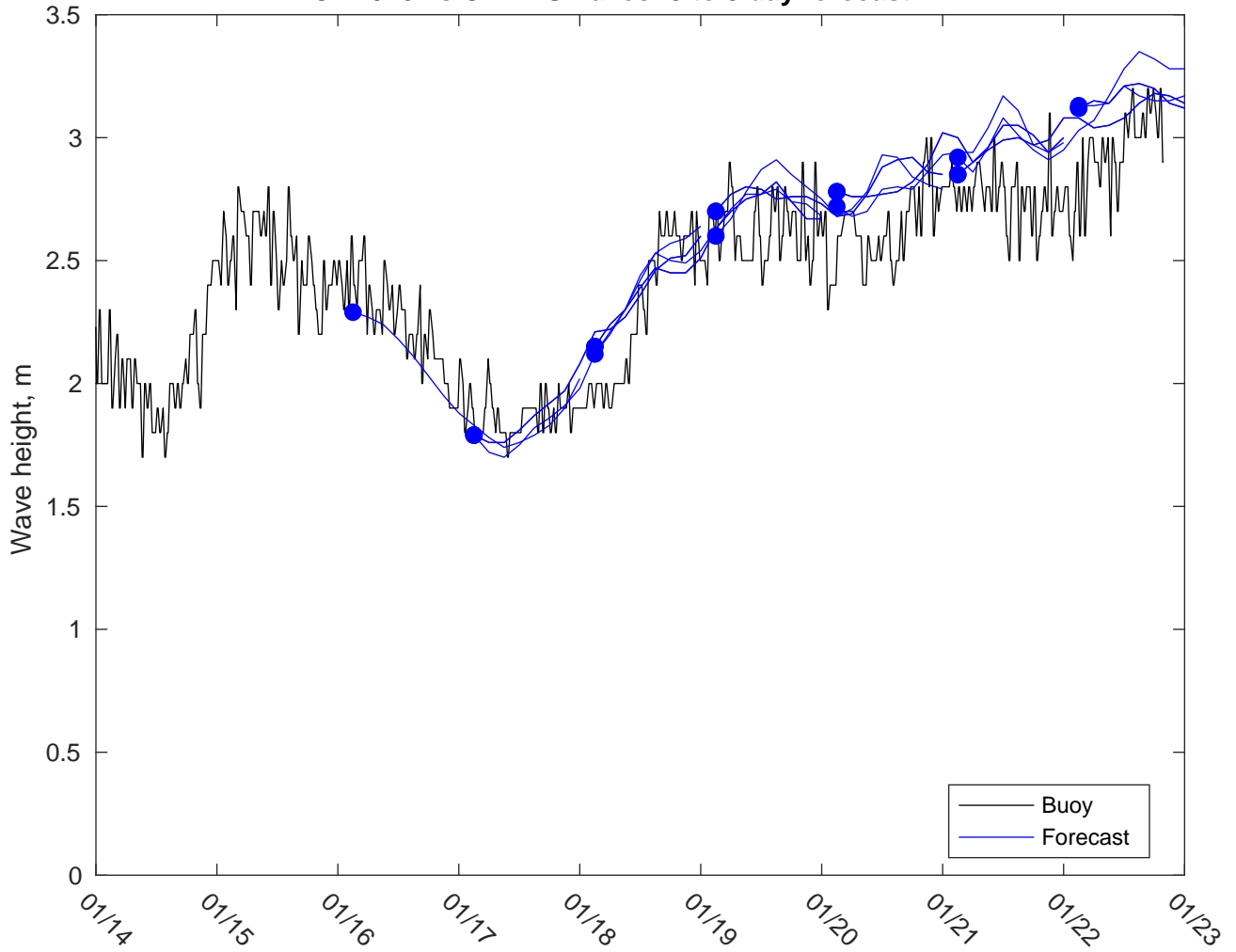
NDBC 41040 vs CMEMSWaves: 3 to 5 day forecast
