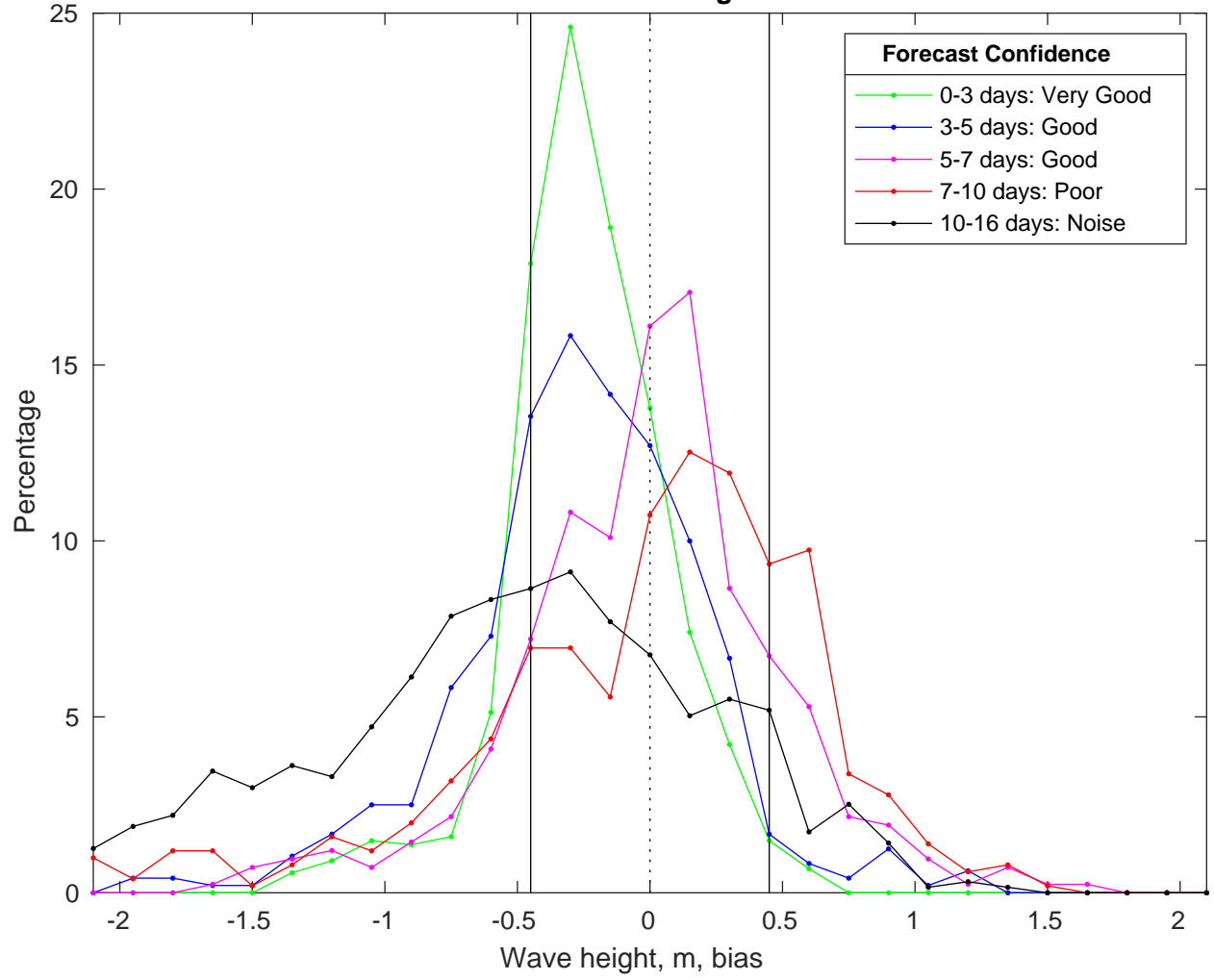
NDBC 42092 vs GFSWaves Bias Histogram: 22-Jan-2025
