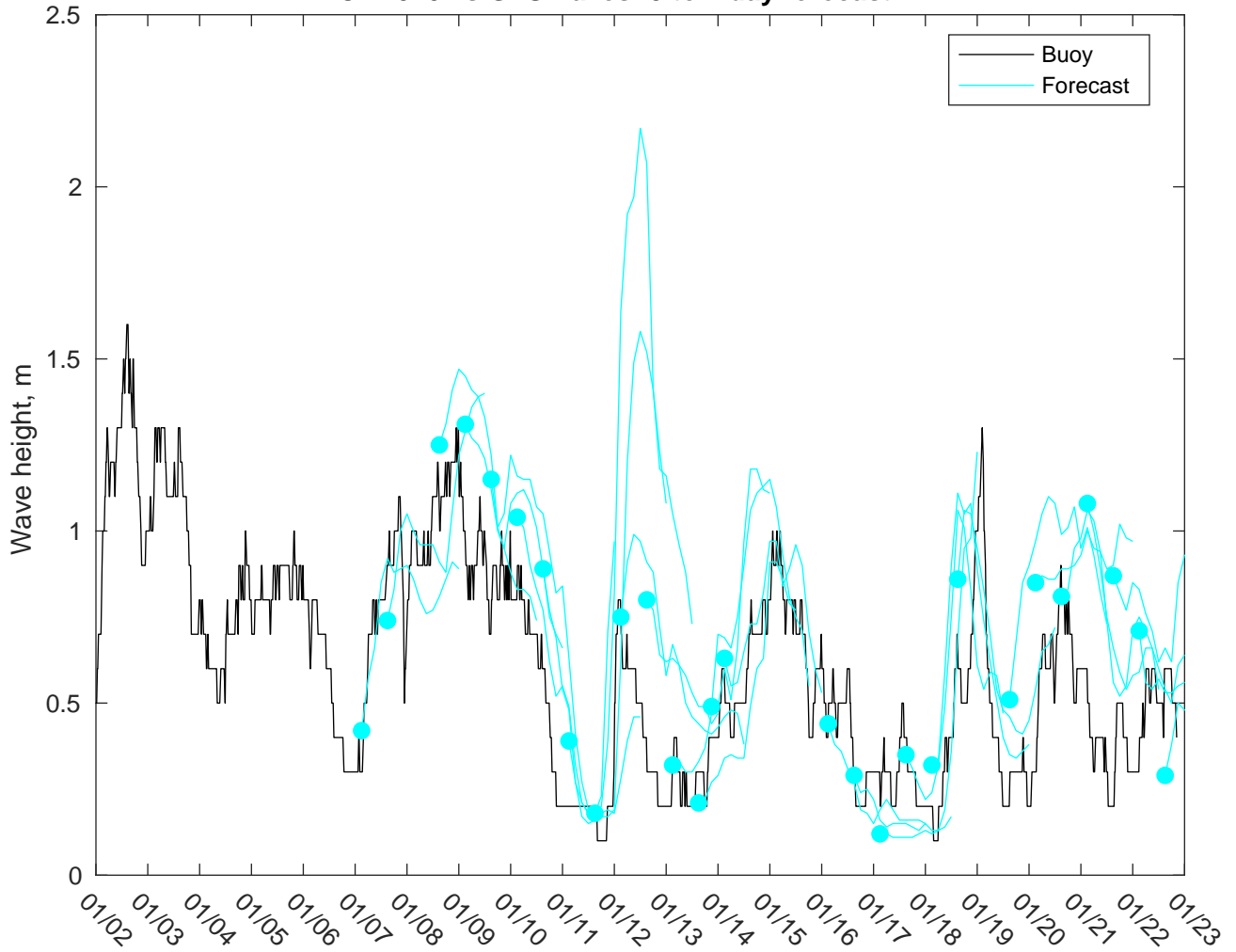
NDBC 44020 vs GFSWaves: 5 to 7 day forecast
