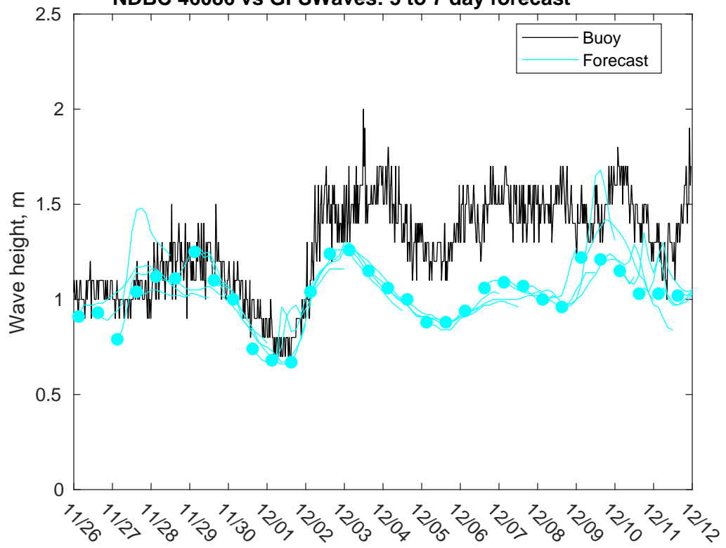
NDBC 46086 vs GFSWaves: 5 to 7 day forecast
