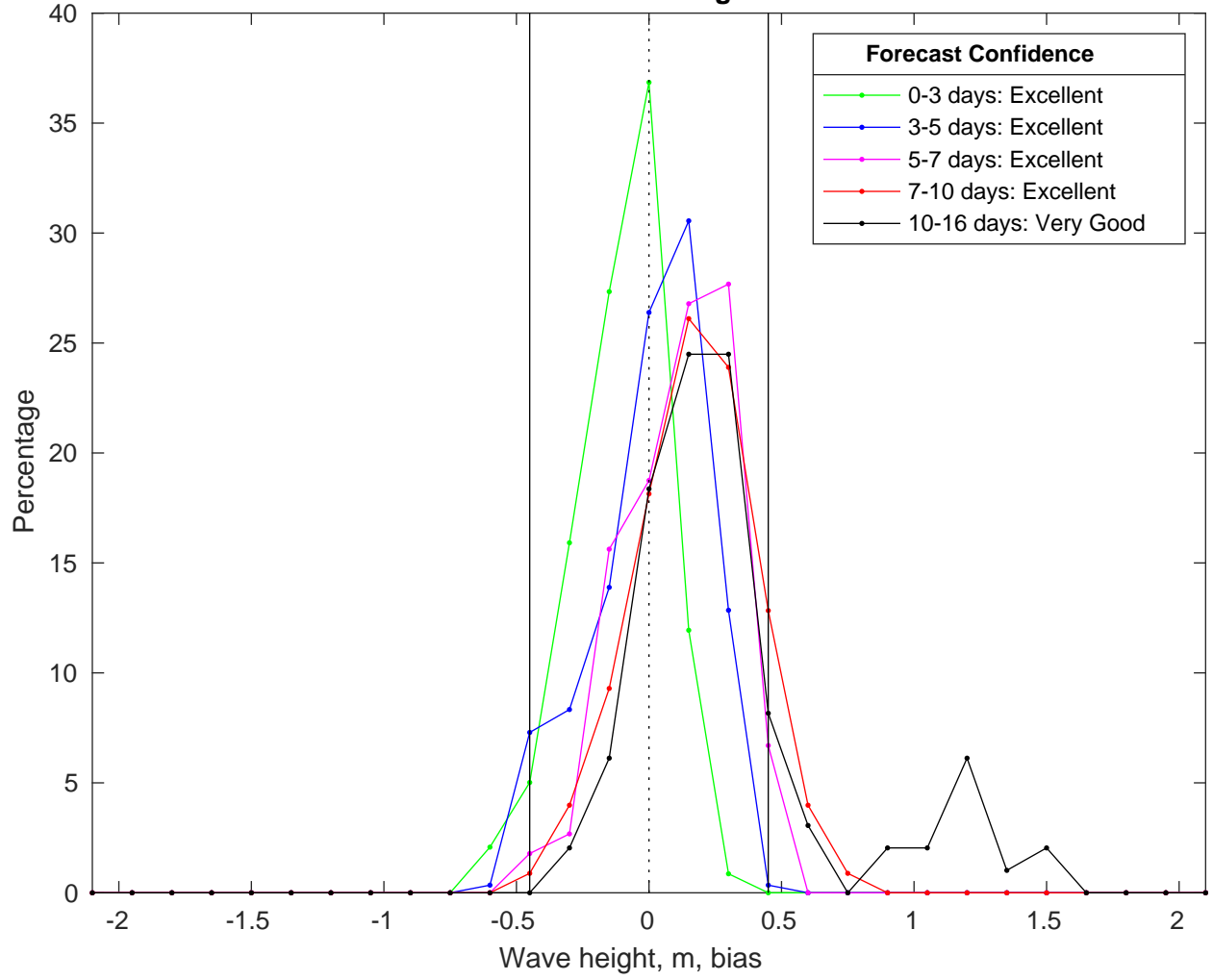
NDBC 52211 vs GFSWaves Bias Histogram: 22-Jan-2025
