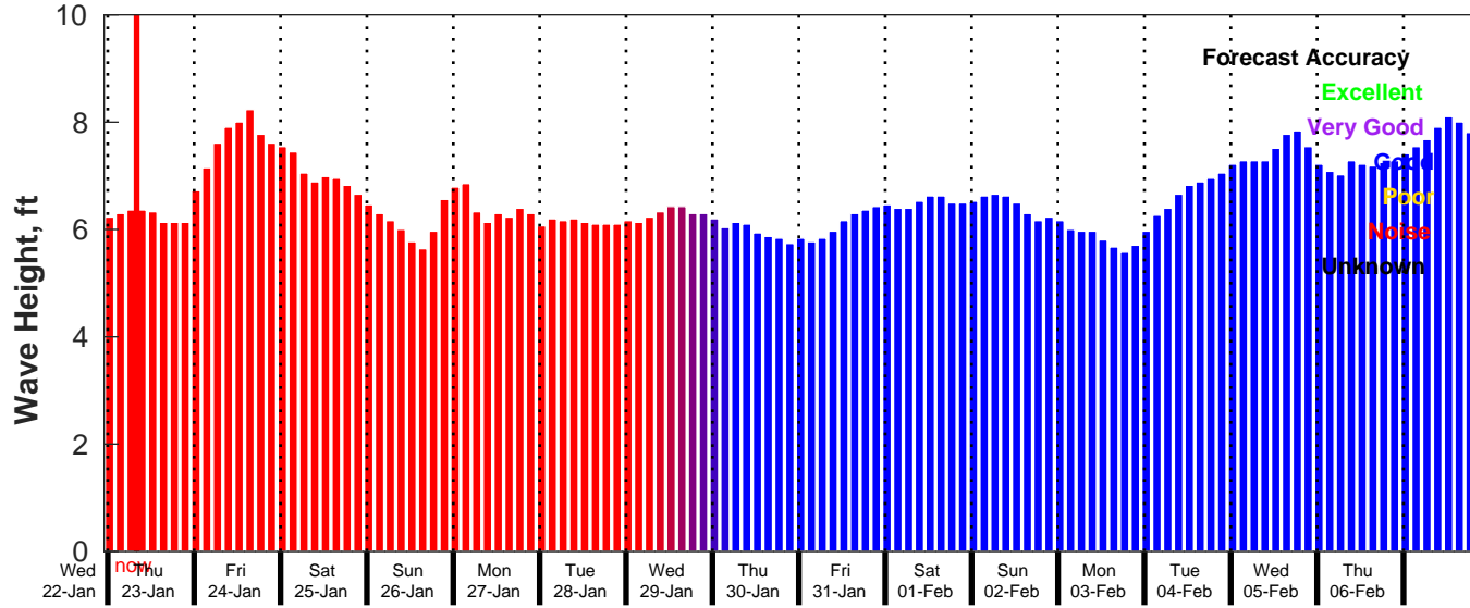
GFS Wave Forecast for NDBC 52213 from 22-Jan-2025 23:00:00 to 07-Feb-2025 23:00:00
