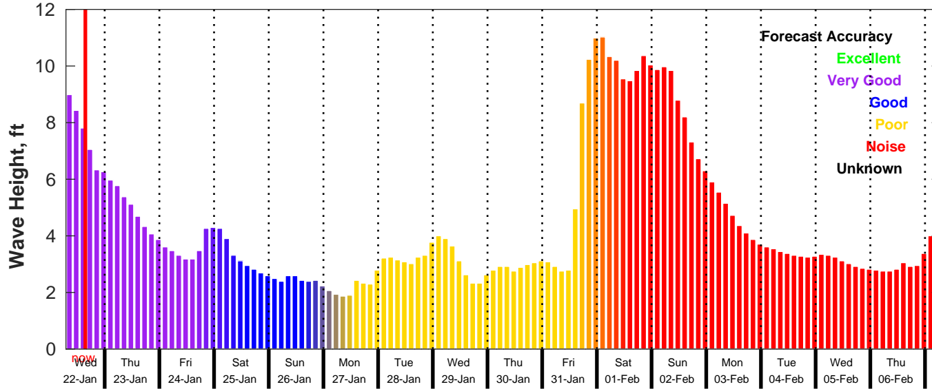
GFS Wave Forecast for NDBC 41004 from 22-Jan-2025 07:00:00 to 07-Feb-2025 07:00:00
