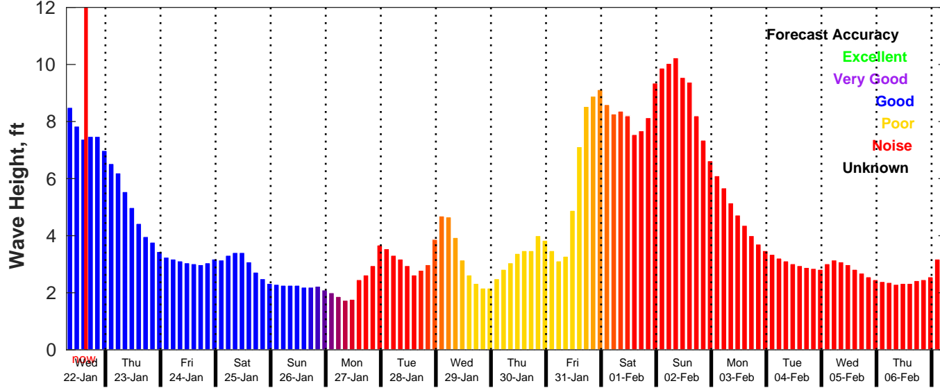
GFS Wave Forecast for NDBC 41013 from 22-Jan-2025 07:00:00 to 07-Feb-2025 07:00:00
