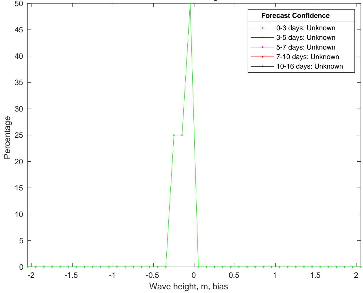
NDBC 42002 vs GFSWaves Bias Histogram: 07-Oct-2024
