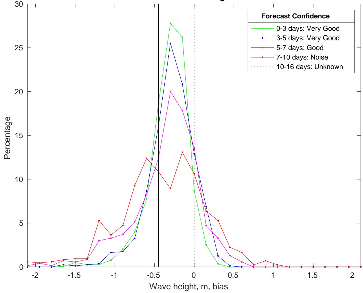
NDBC 42035 vs CMEMSWaves Bias Histogram: 22-Jan-2025
