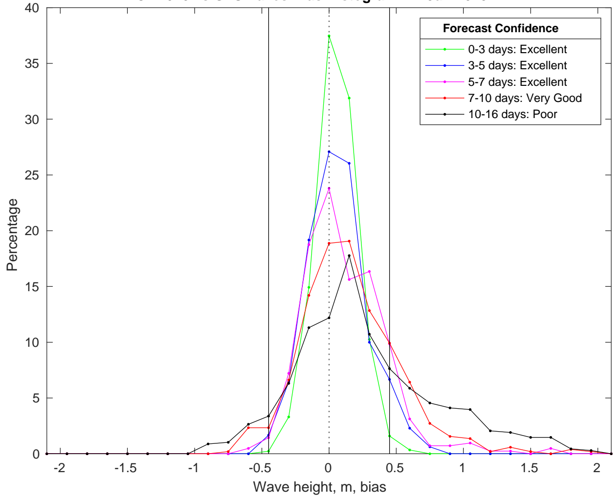
NDBC 44020 vs GFSWaves Bias Histogram: 22-Jan-2025
