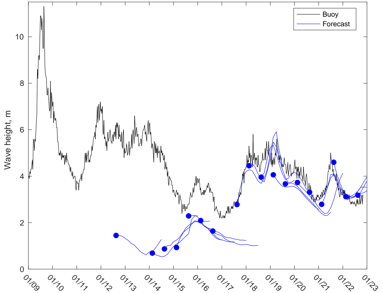
NDBC 46246 vs GFSWaves: 3 to 5 day forecast
