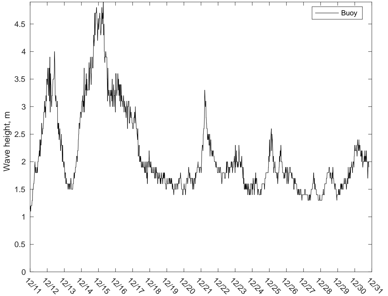
NDBC 41002 vs CMEMSWaves: 10 to 16 day forecast
