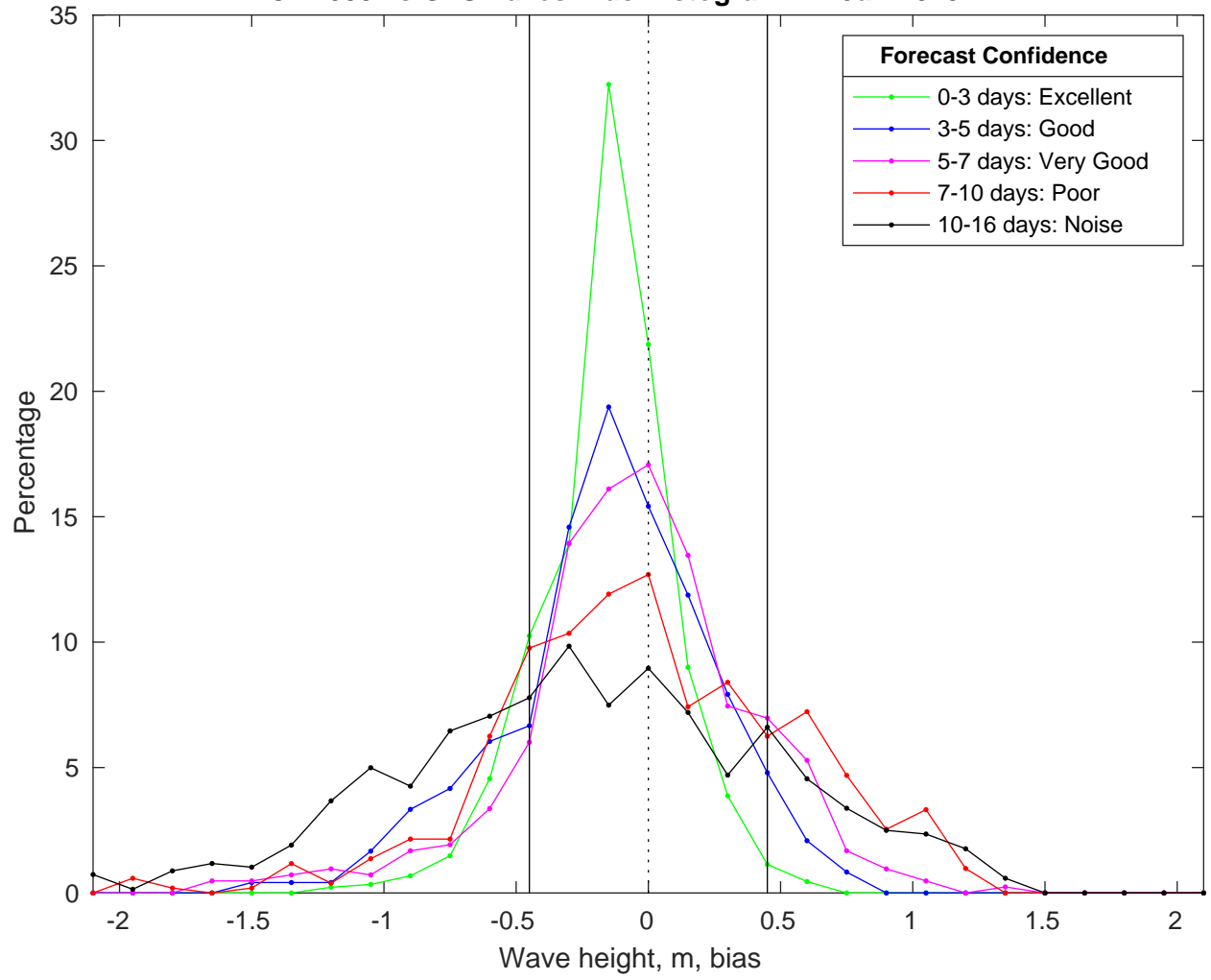
NDBC 42035 vs GFSWaves Bias Histogram: 22-Jan-2025
