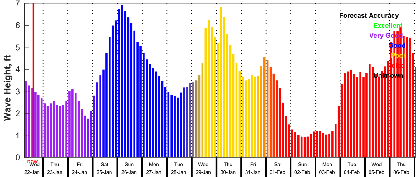
GFS Wave Forecast for NDBC 42092 from 22-Jan-2025 06:00:00 to 07-Feb-2025 06:00:00
