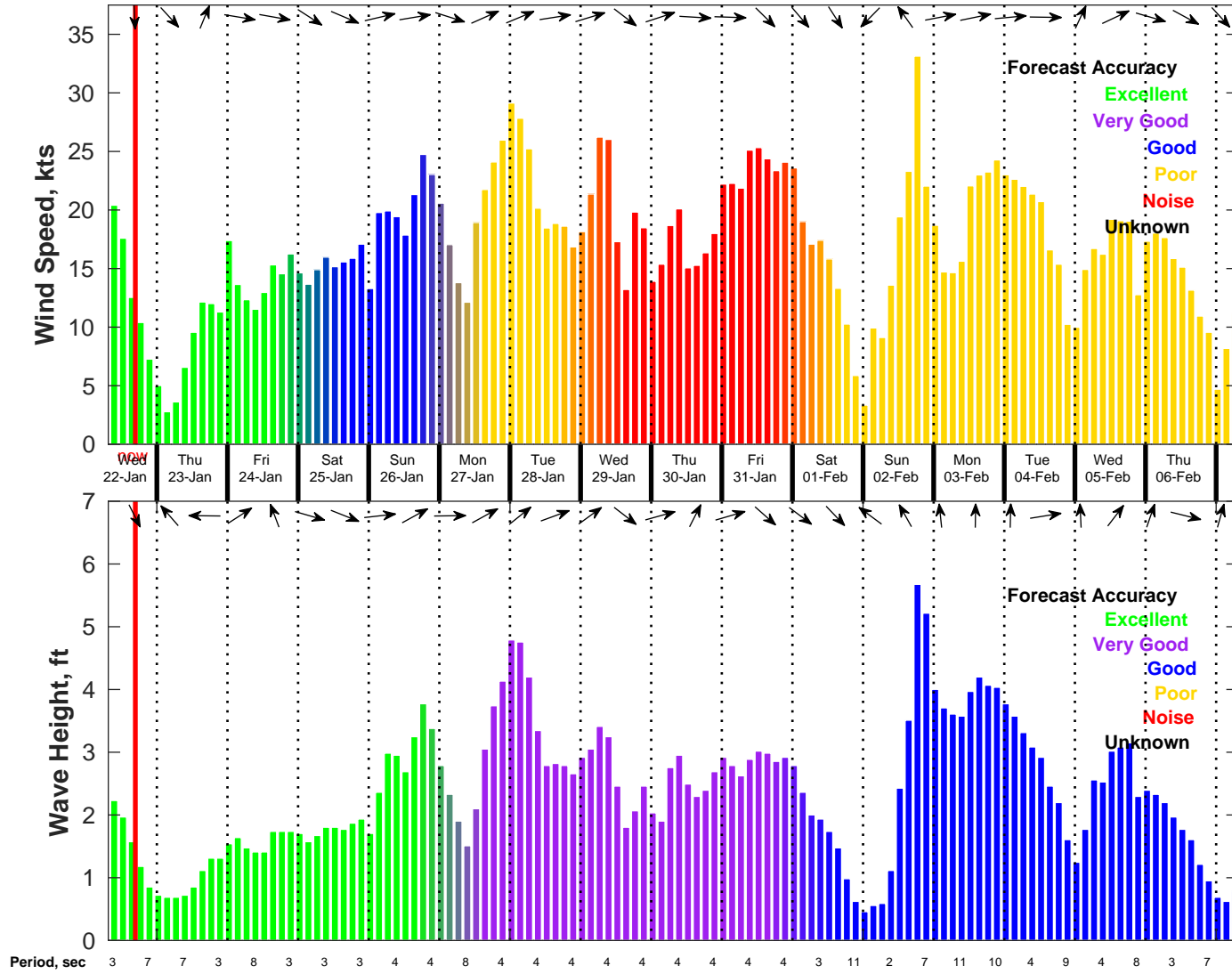
Wind & Wave Forecast for NDBC 44020 from 22-Jan-2025 08:00:00 to 07-Feb-2025 08:00:00
