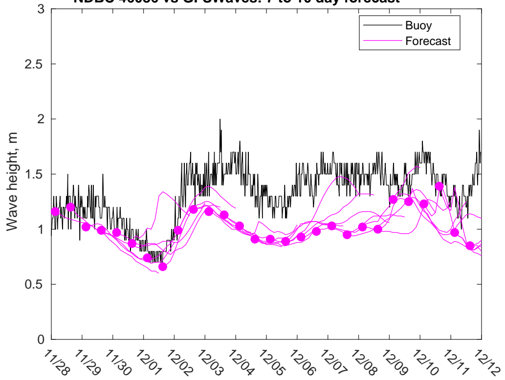
NDBC 46086 vs GFSWaves: 7 to 10 day forecast
