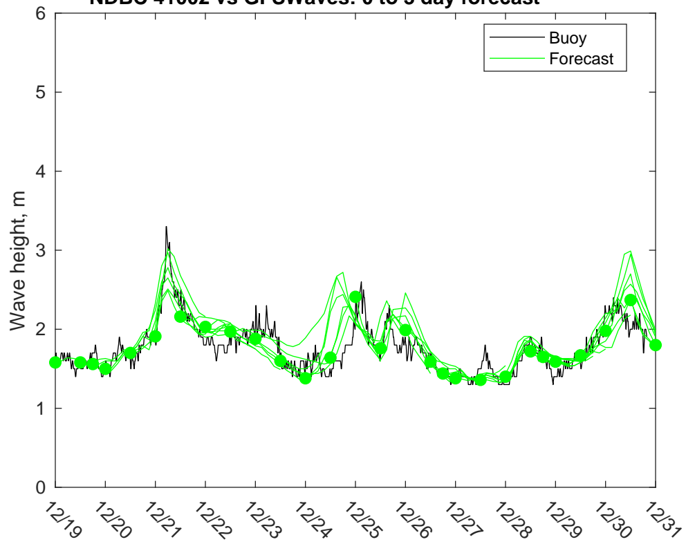
NDBC 41002 vs GFSWaves: 0 to 3 day forecast
