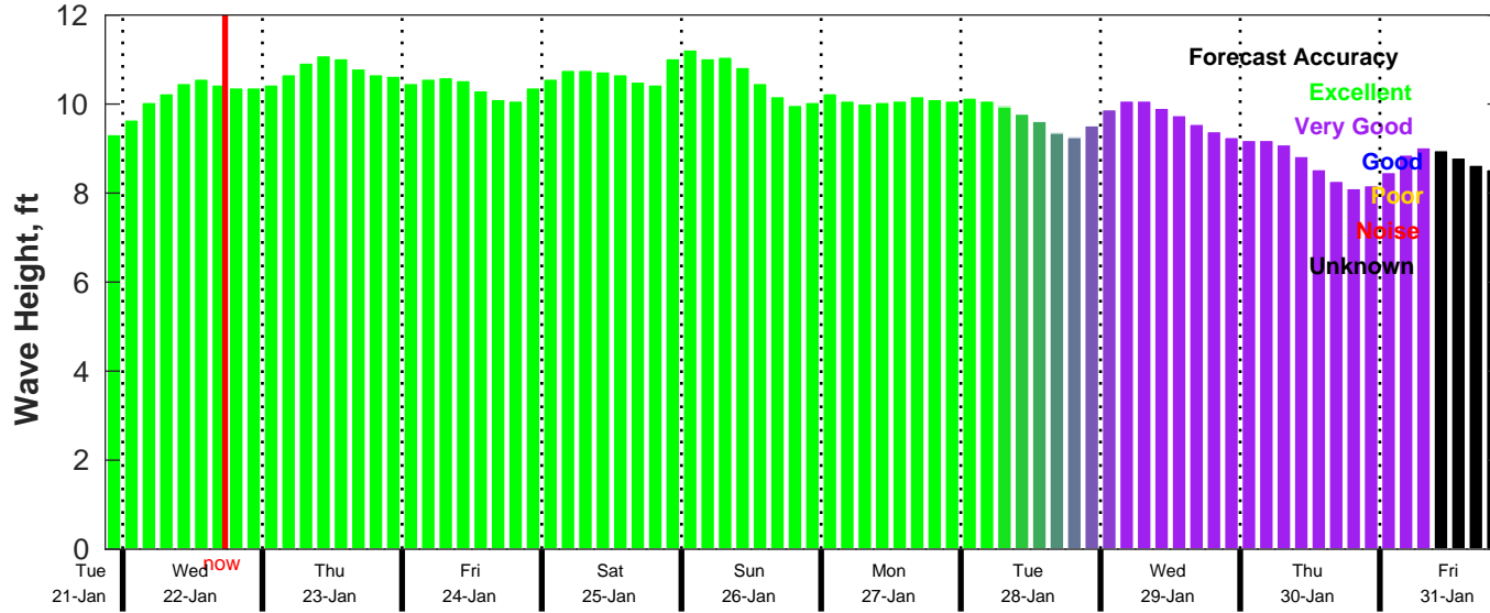
CMEMS Wave Forecast for NDBC 41040 from 21-Jan-2025 21:00:00 to 31-Jan-2025 21:00:00
