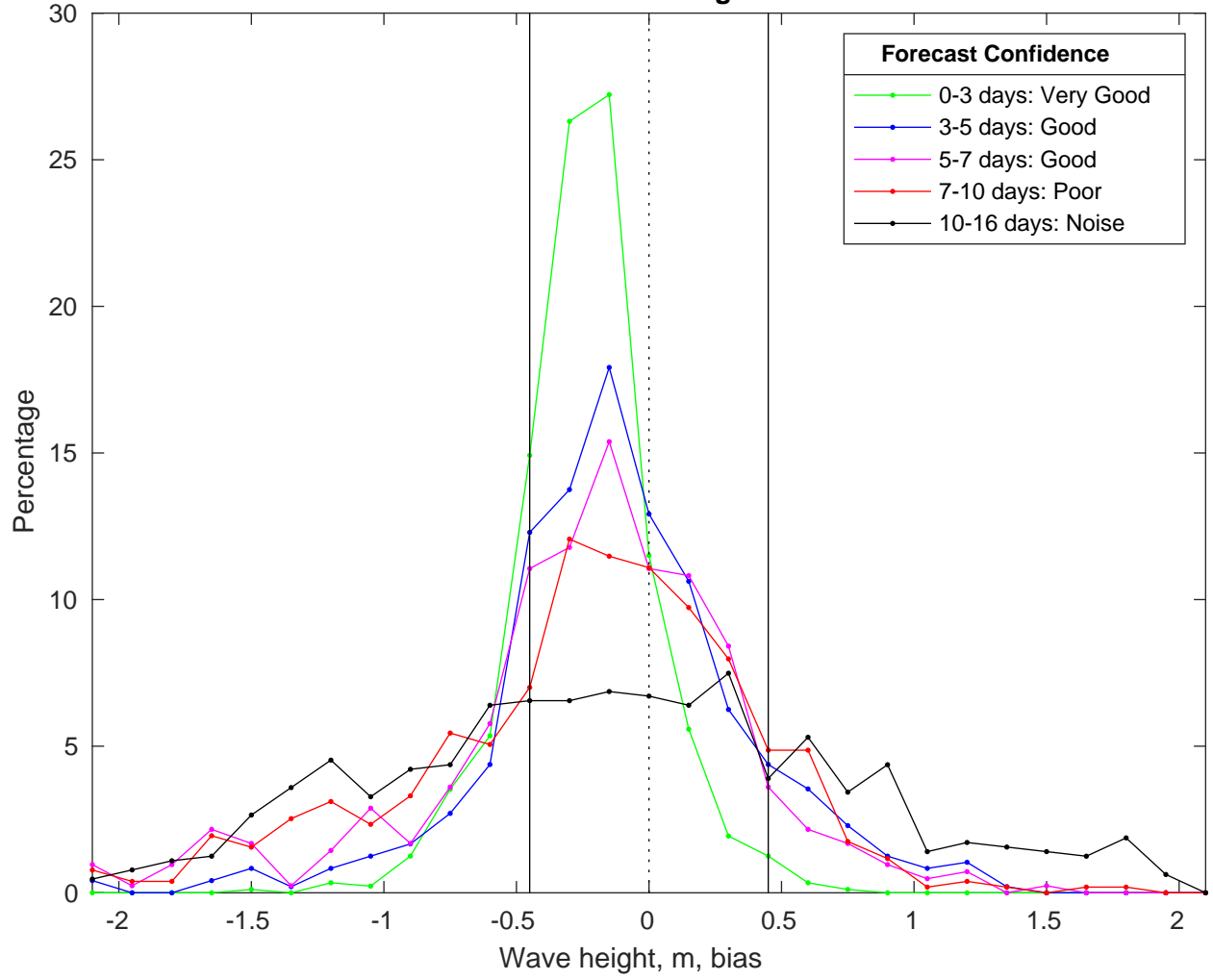
NDBC 42036 vs GFSWaves Bias Histogram: 22-Jan-2025
