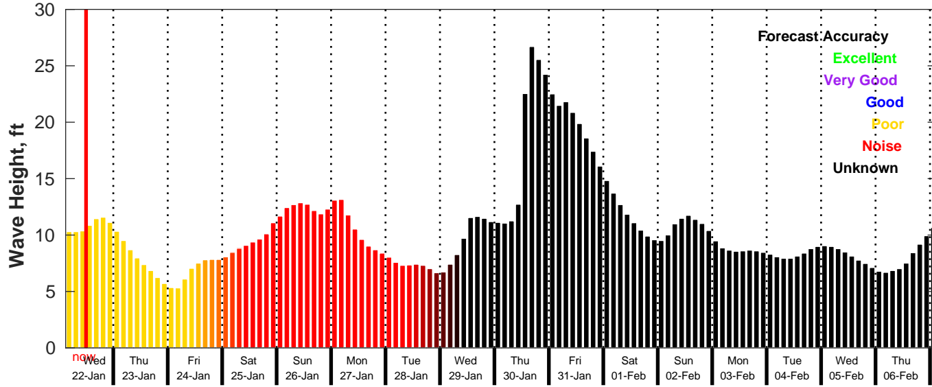
GFS Wave Forecast for NDBC 46246 from 22-Jan-2025 03:00:00 to 07-Feb-2025 03:00:00
