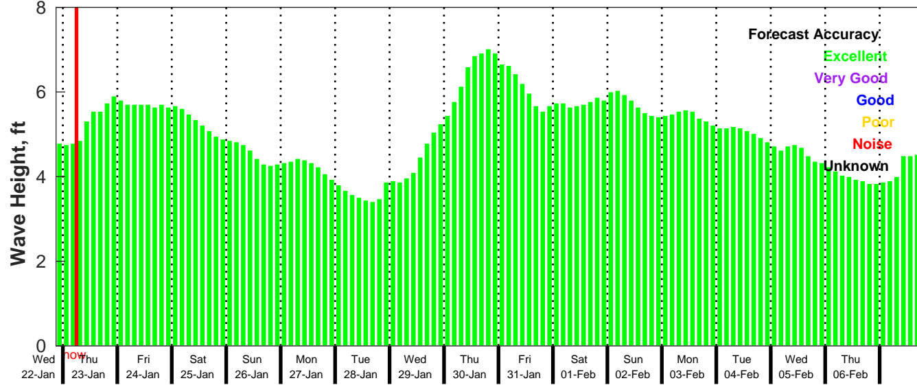
GFS Wave Forecast for NDBC 52212 from 22-Jan-2025 21:00:00 to 07-Feb-2025 21:00:00
