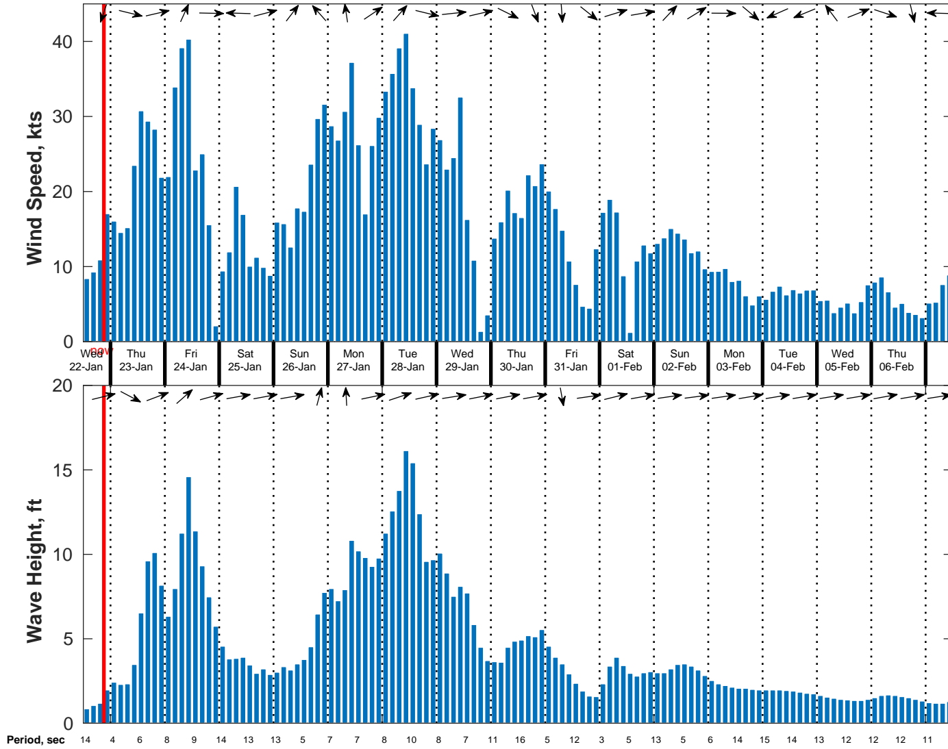
Wind & Wave Forecast for NDBC 62305 from 22-Jan-2025 12:00:00 to 07-Feb-2025 12:00:00
