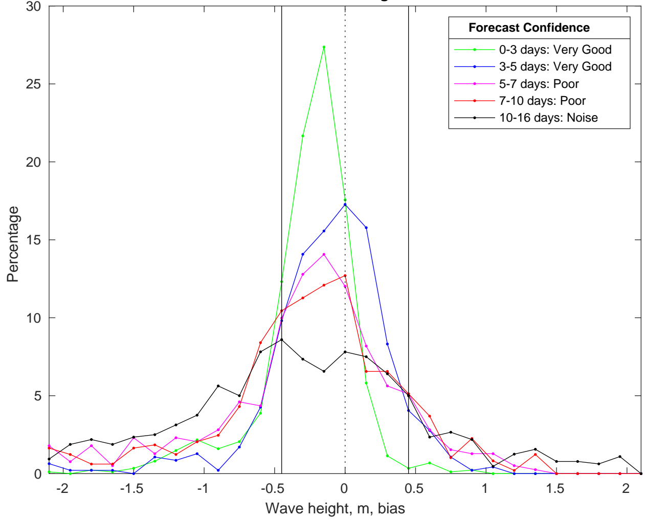
NDBC 42040 vs GFSWaves Bias Histogram: 22-Jan-2025
