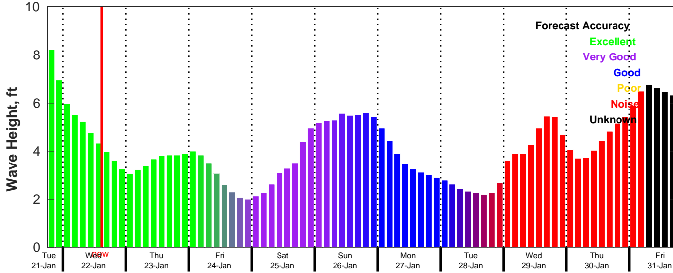
CMEMS Wave Forecast for NDBC 42092 from 21-Jan-2025 18:00:00 to 31-Jan-2025 18:00:00
