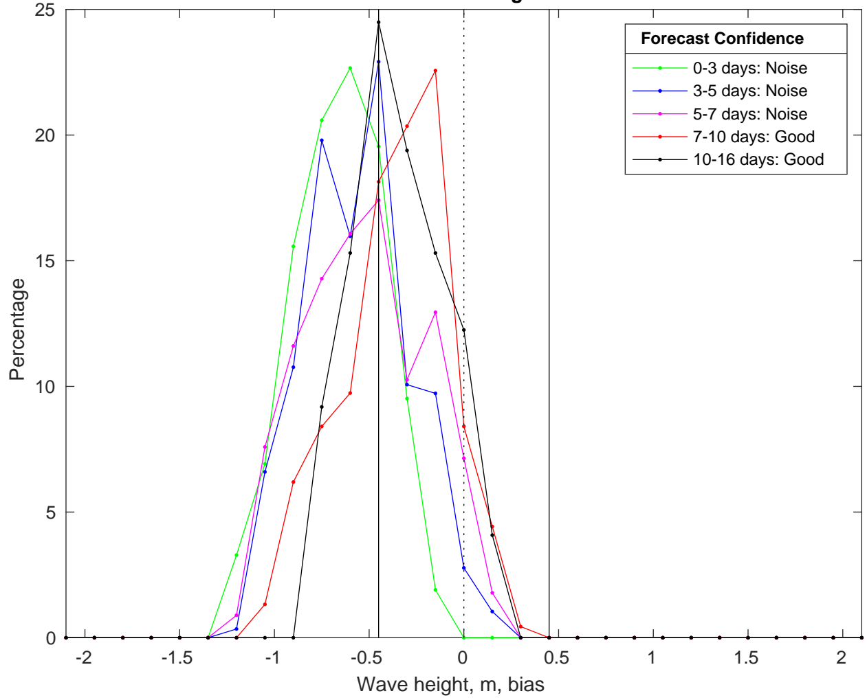
NDBC 52213 vs GFSWaves Bias Histogram: 22-Jan-2025
