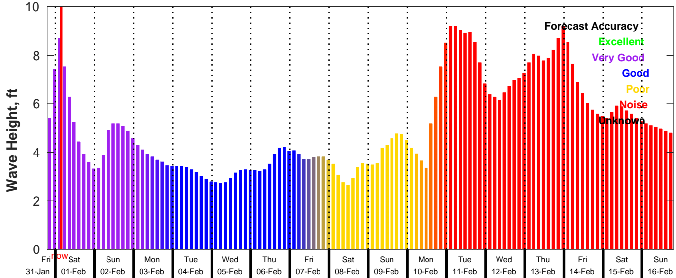
GFS Wave Forecast for NDBC 41004 from 31-Jan-2025 19:00:00 to 16-Feb-2025 19:00:00
