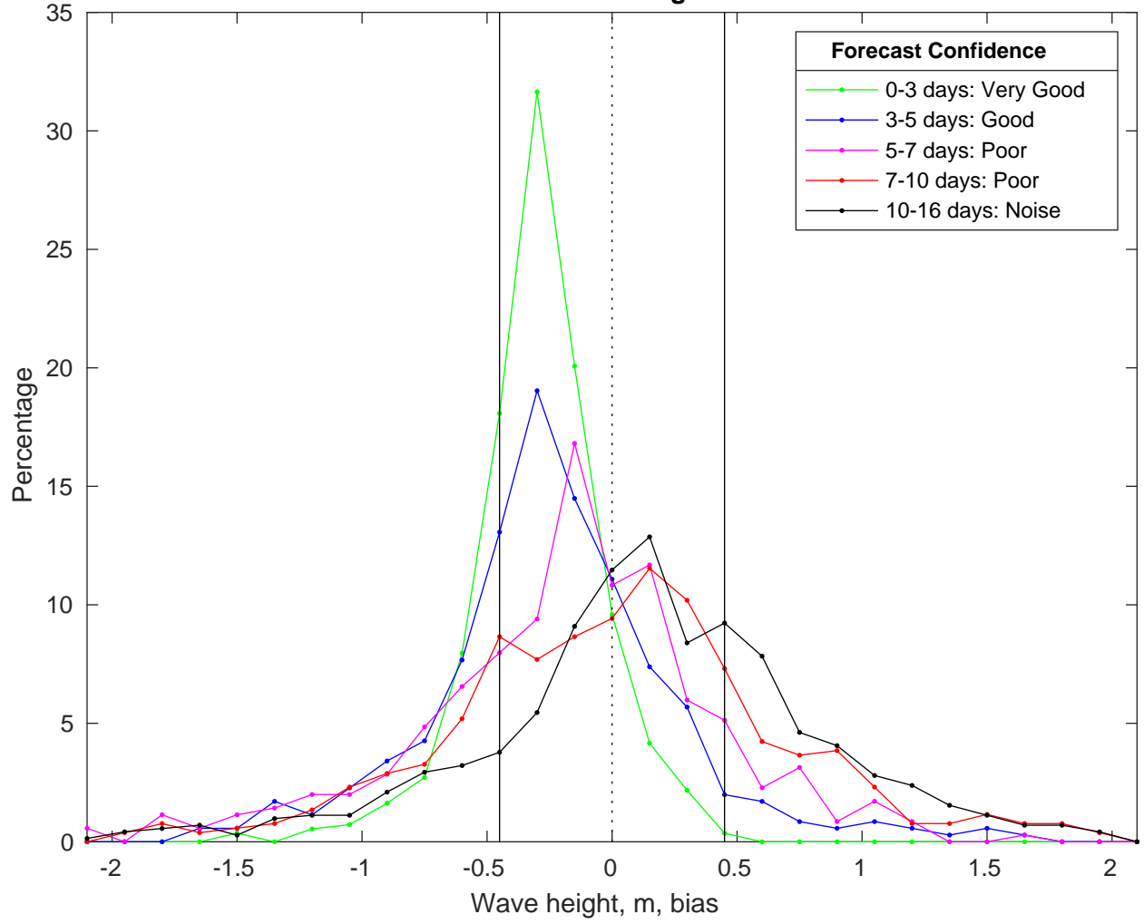
NDBC 41013 vs GFSWaves Bias Histogram: 01-Feb-2025
