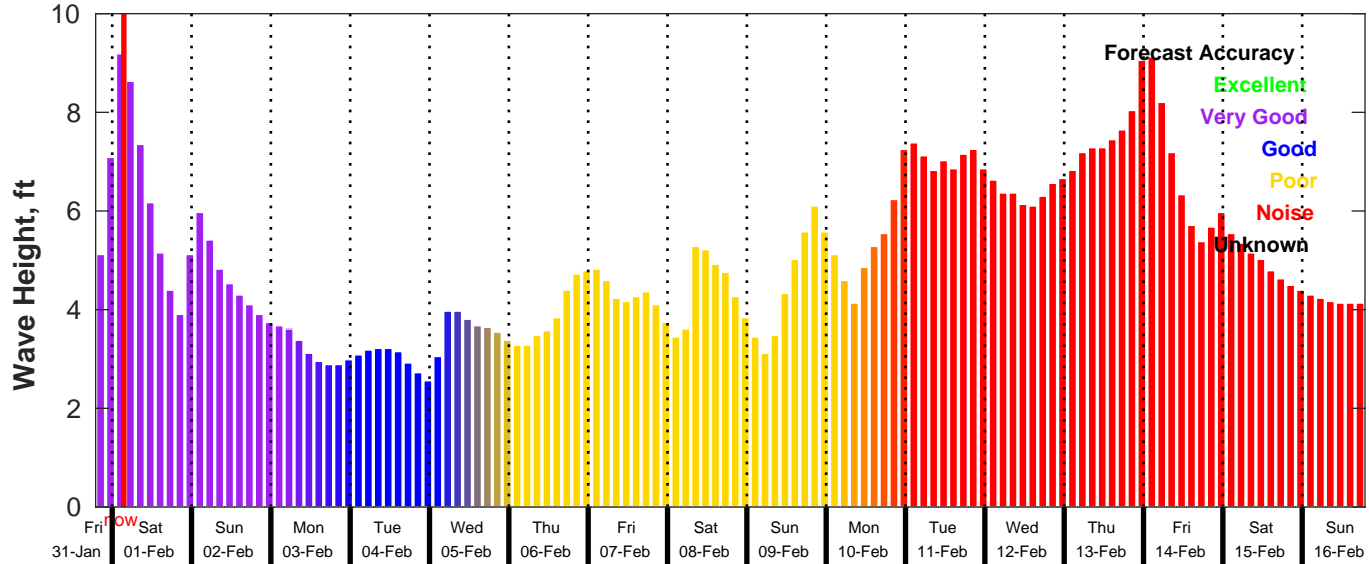
GFS Wave Forecast for NDBC 41013 from 31-Jan-2025 19:00:00 to 16-Feb-2025 19:00:00
