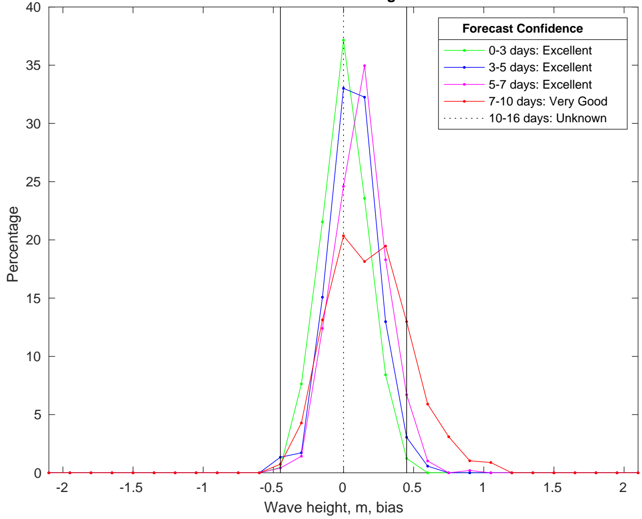
NDBC 41040 vs CMEMSWaves Bias Histogram: 01-Feb-2025
