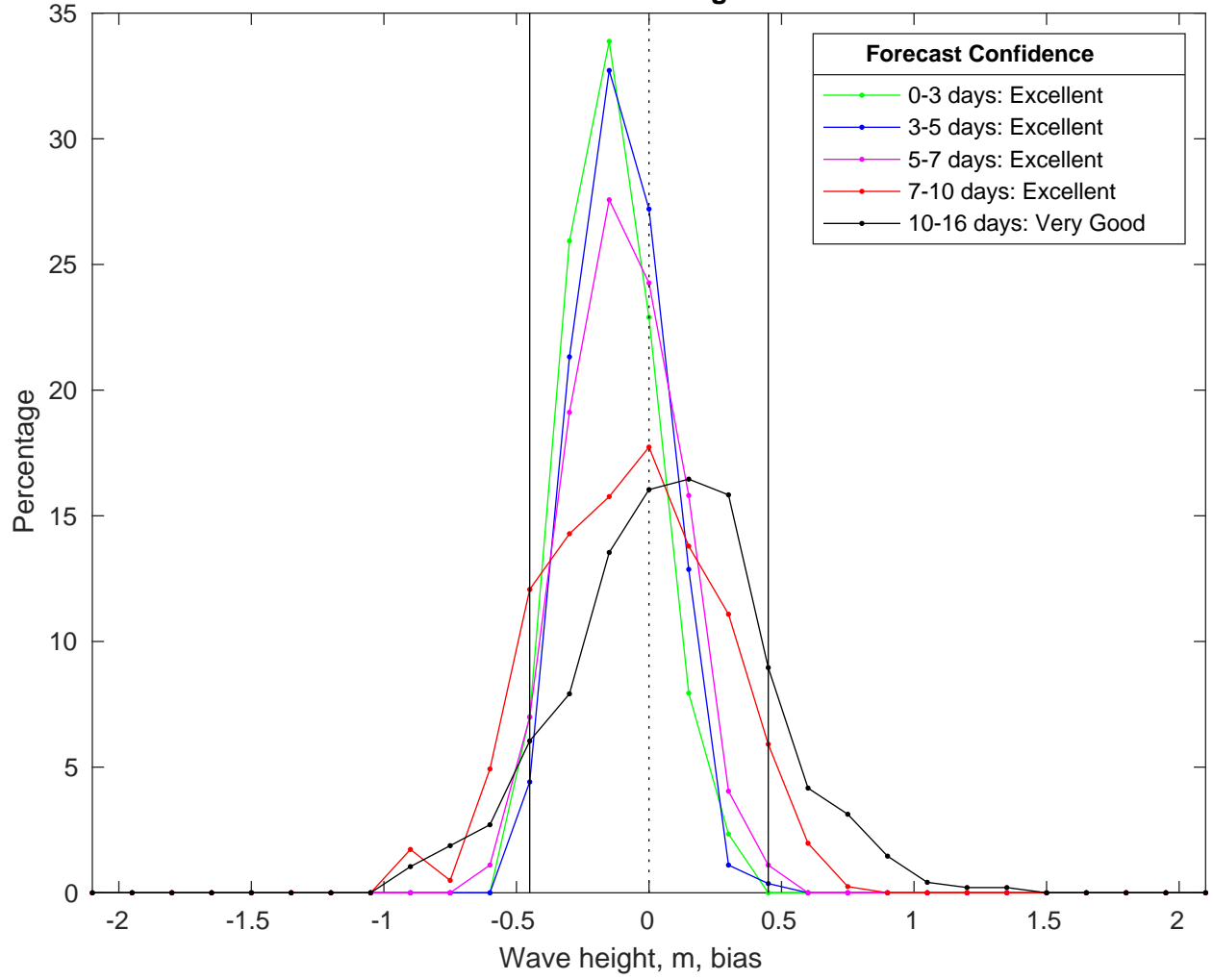
NDBC 41040 vs GFSWaves Bias Histogram: 01-Feb-2025
