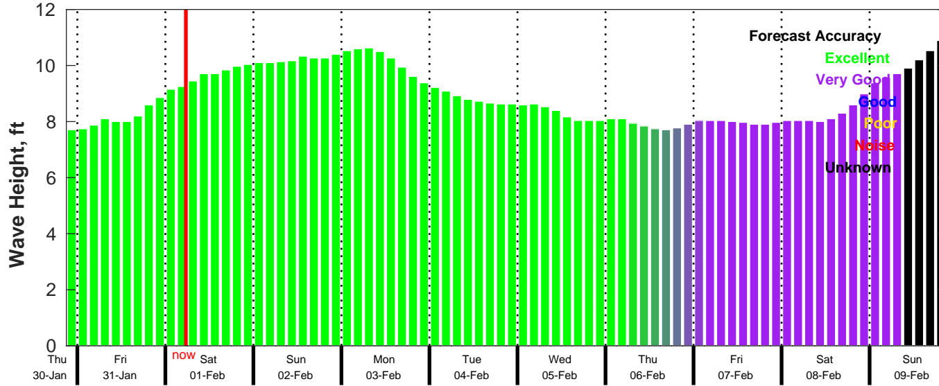
CMEMS Wave Forecast for NDBC 41040 from 30-Jan-2025 21:00:00 to 09-Feb-2025 21:00:00
