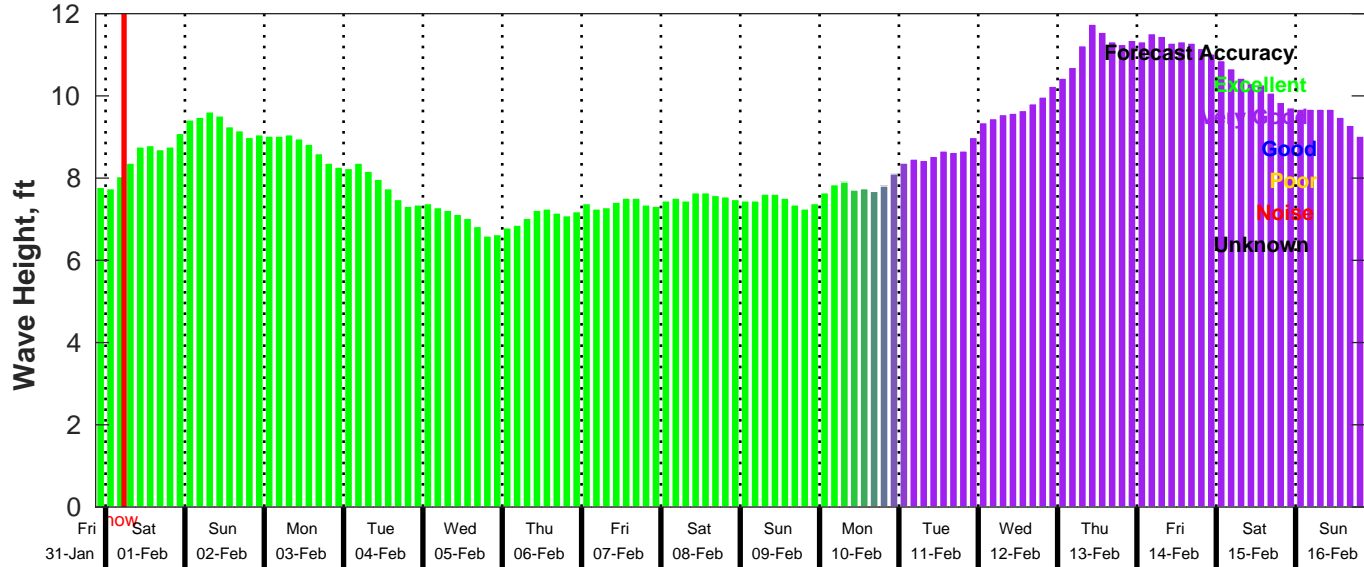
GFS Wave Forecast for NDBC 41040 from 31-Jan-2025 21:00:00 to 16-Feb-2025 21:00:00
