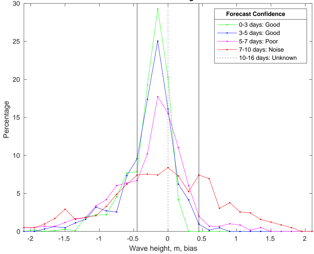
NDBC 42020 vs CMEMSWaves Bias Histogram: 01-Feb-2025
