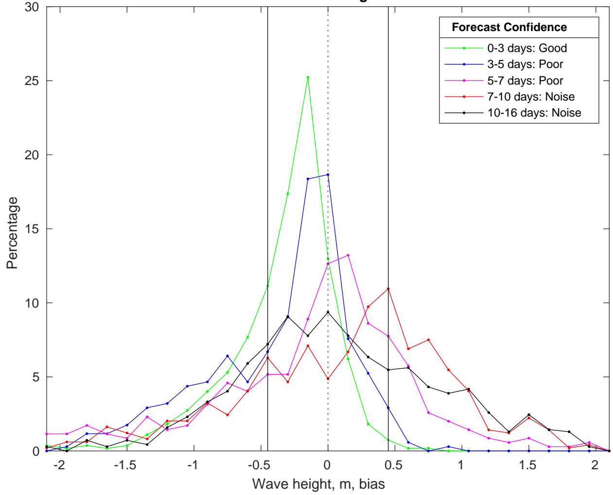
NDBC 42020 vs GFSWaves Bias Histogram: 01-Feb-2025
