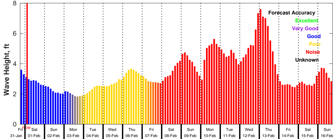
GFS Wave Forecast for NDBC 42020 from 31-Jan-2025 18:00:00 to 16-Feb-2025 18:00:00
