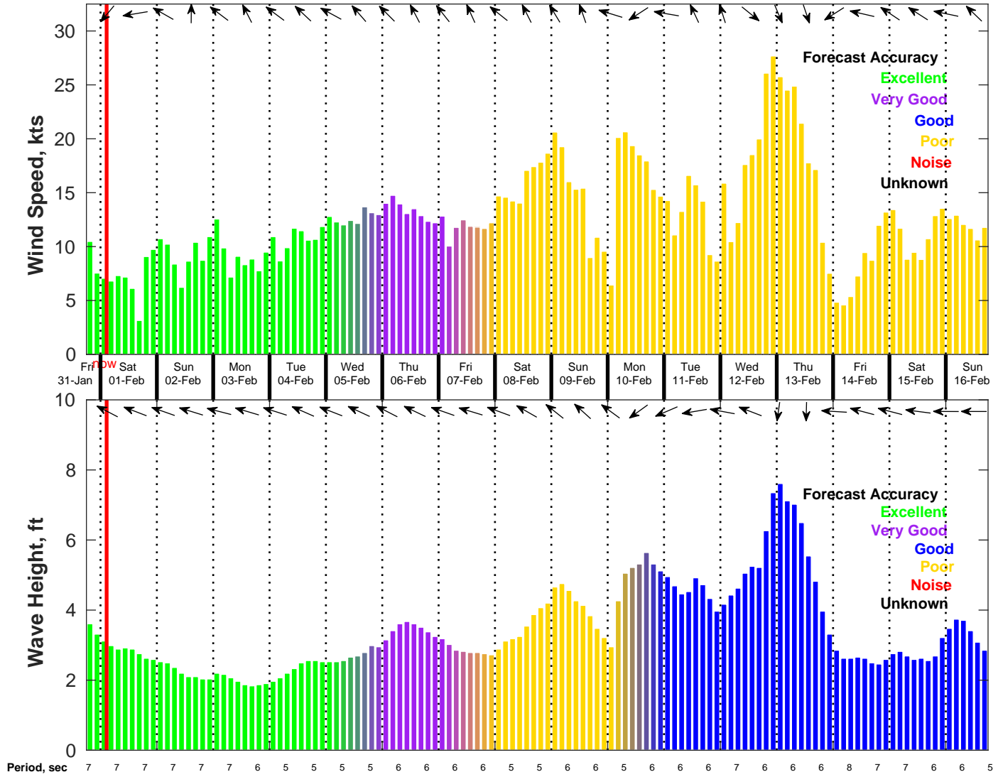
Wind & Wave Forecast for NDBC 42020 from 31-Jan-2025 18:00:00 to 16-Feb-2025 18:00:00
