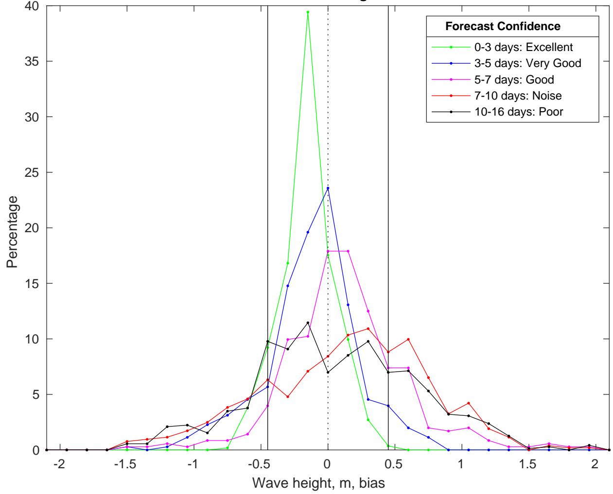
NDBC 42035 vs GFSWaves Bias Histogram: 01-Feb-2025
