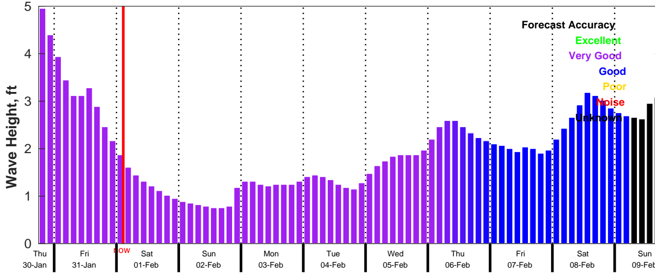
CMEMS Wave Forecast for NDBC 42035 from 30-Jan-2025 18:00:00 to 09-Feb-2025 18:00:00
