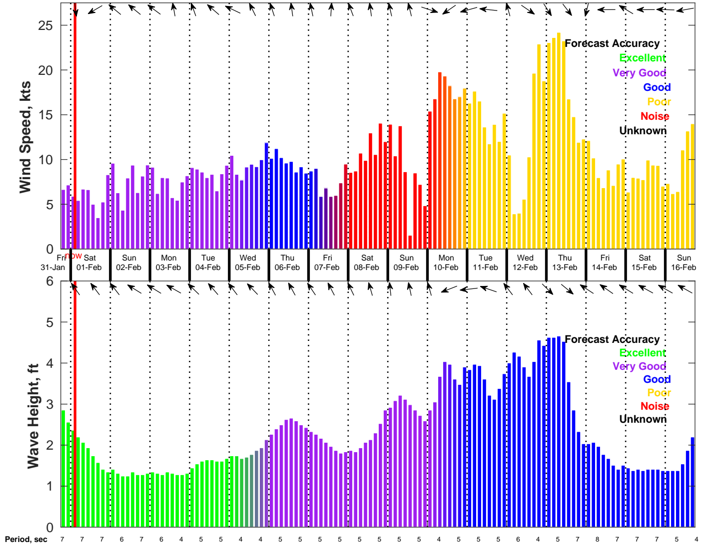
Wind & Wave Forecast for NDBC 42035 from 31-Jan-2025 18:00:00 to 16-Feb-2025 18:00:00
