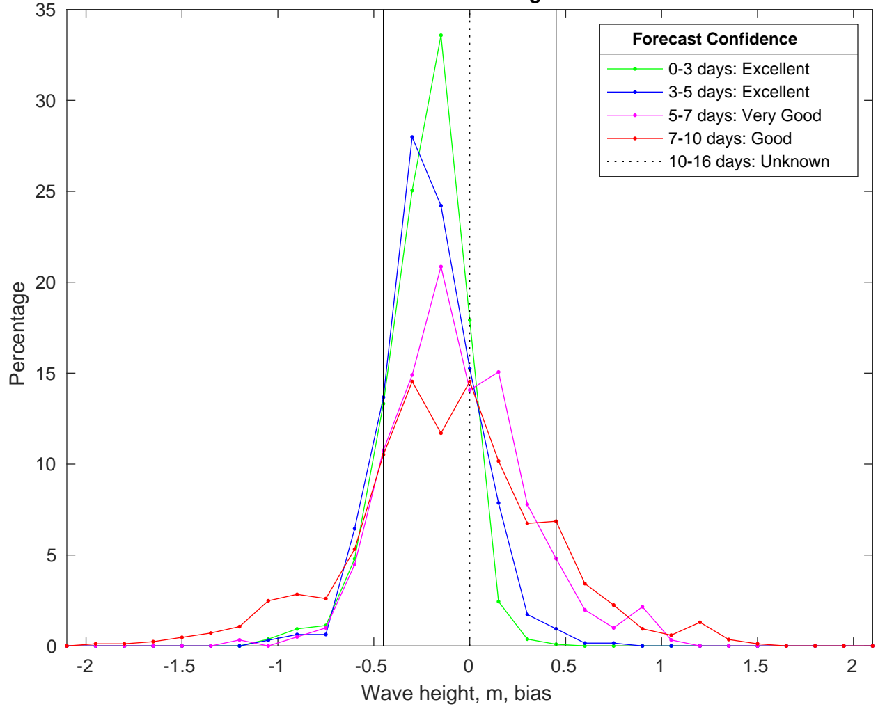
NDBC 42036 vs CMEMSWaves Bias Histogram: 01-Feb-2025
