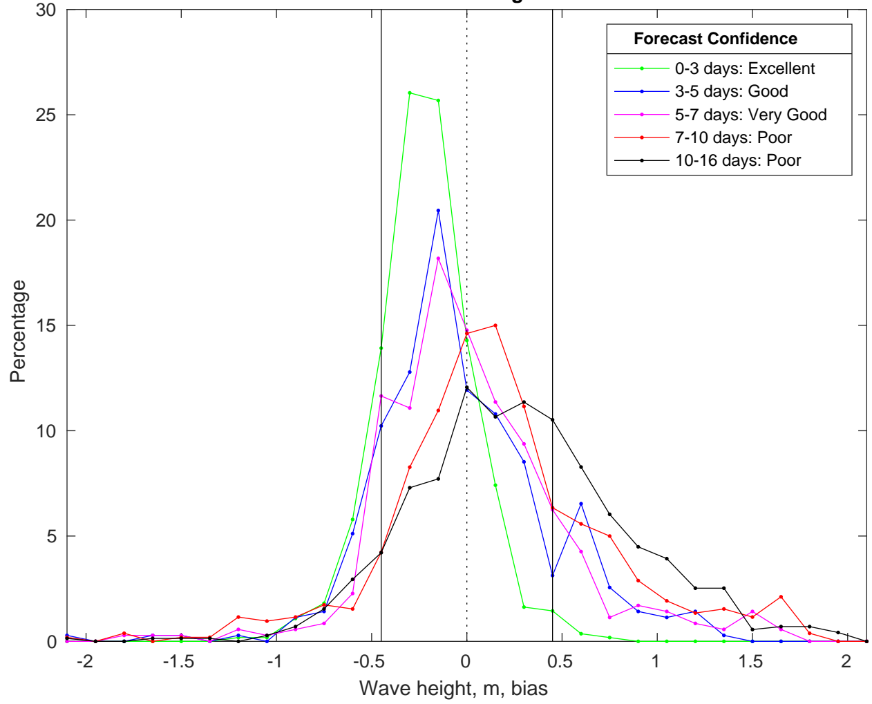
NDBC 42036 vs GFSWaves Bias Histogram: 01-Feb-2025
